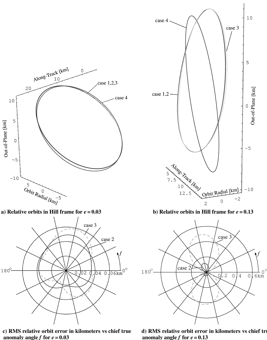
Fig. 3 Comparison of the linearized relative orbit solutions for cases 1–4 with e = 0.03 and e = 0.13 .
